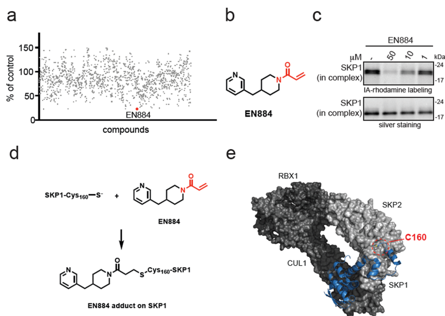
Figure 1. Discovery of a covalent SKP1 recruiter. (a) Gel-based ABPP screening of a cysteine-reactive covalent ligand library (50 \mu\text{M} ) against a rhodamine-functionalized iodoacetamide (IA-rhodamine) labeling of pure SKP1 protein in the SKP1-FBXO7-CUL1-RBX1 complex. Individual compound values are noted as percent of labeling compared to that of DMSO vehicle control. EN884 was the top hit that showed the most inhibition of probe labeling. Structures of compounds screened and screening data can be found in Table S1. (b) Structure of EN884 with the cysteine-reactive acrylamide warhead in red. (c) Gel-based ABPP of EN884 competition against IA-rhodamine labeling. Pure SKP1 in the SKP1-FBXO7-CUL1-RBX1 complex was preincubated with EN884 1 h prior to labeling with IA-rhodamine (100 nM) for 30 min after which the proteins were separated by SDS/PAGE and visualized by in-gel fluorescence. Protein loading was assessed by silver staining. (d) Mass spectrometry analysis of EN884 modification on SKP1 shown in Figure S2a within the SKP1-FBXO7-CUL1-RBX1 complex from incubation of the complex with EN884 (50 \mu\text{M} ) for 1 h, followed by MS/MS analysis of tryptic digests revealed one site of EN884 modification on SKP1 at C160. (e) Shown is the location in the circle of SKP1 C160 in the CUL1 complex with SKP1 in blue, in complex with SKP2, RBX1, and CUL1. Shown is an SCF complex model derived from superimposing the crystal structures of Skp1-Skp2-Cks1 with p27 peptide (PDB ID: 2AST) and Cul1-Rbx1-Skp1-Skp2 (PDB ID: 1LDK). SKP1 is shown as the blue ribbon structure, SKP2 in light gray, and RBX1-CUL1 in dark gray. The C160 side-chain is shown in yellow and circled in red. Data shown in (b) are from n = 3 biologically independent replicates per group.
