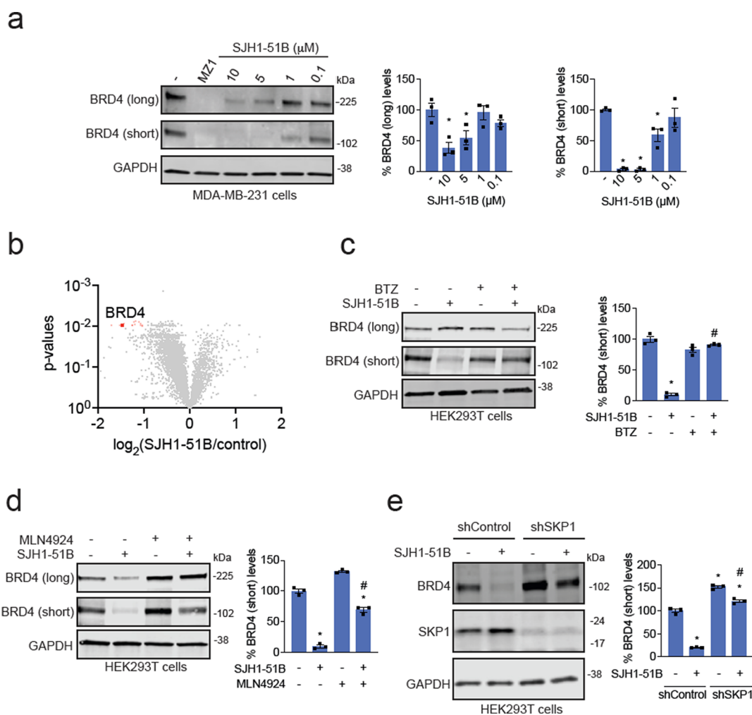
Figure 4. Characterization of BRD4 degrader. (a) BRD4 degradation in MDA-MB-231 cells. MDA-MB-231 cells were treated with DMSO vehicle, MZ1 (1 \mu M), or SJH1-51B for 24 h. The long and short isoforms of BRD4 and loading control GAPDH were assessed by Western blotting, and bands were quantified by densitometry and normalized to GAPDH. (b) TMT-based quantitative proteomic profiling of SJH1-51B in MDA-MB-231 cells. MDA-MB-231 cells were treated with DMSO vehicle or SJH1-51B (10 \mu M) for 24 h. Proteomics data can be found in Table S4. (c, d) Proteasome and NEDDylation-dependence of BRD4 degradation. HEK293T cells were pretreated with DMSO vehicle or bortezomib (1 \mu M) in (c) or MLN4924 (1 \mu M) in (d) for 1 h prior to treatment of cells with DMSO vehicle or SJH1-51B (10 \mu M) for 24 h. BRD4 and loading control GAPDH levels were assessed by Western blotting and quantified. (e) Attenuation of BRD4 degradation by SKP1 knockdown. shControl and shSKP1 HEK293T cells were treated with DMSO vehicle or SJH1-51B (5 \mu M) for 24 h. Short BRD4 isoform, SKP1, and loading control GAPDH levels were assessed by Western blotting and quantified. Blots in (a, c, d, e) are representative of n = 3 biologically independent replicates/group. Bar graphs show average \pm sem and individual replicate values of BRD4 levels. Significance is expressed as * p < 0.05 compared to vehicle-treated controls, and # p < 0.05 compared to either SJH1-51B treatment alone in (c, d) or compared to SJH1-51B-treated shControl cells in (e).
